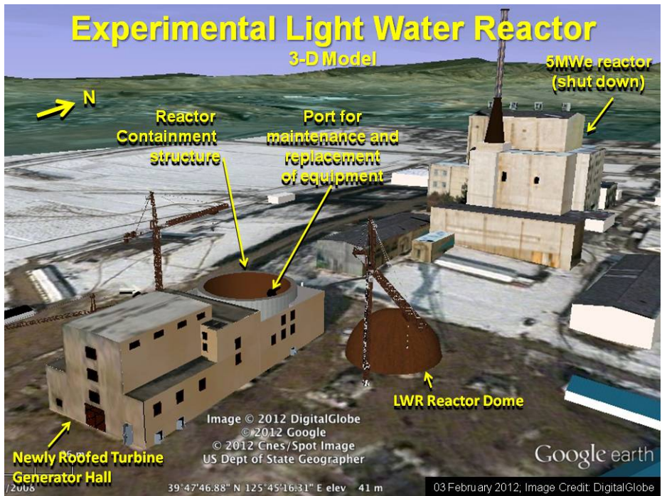
Figure 3 – Three-dimensional model of the light water reactor based on latest satellite images
