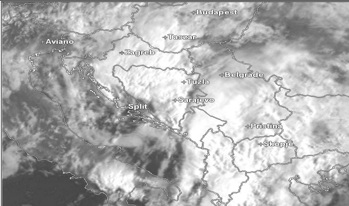
Figure 9 Satellite Image of Typical Weather in Kosovo (U)
