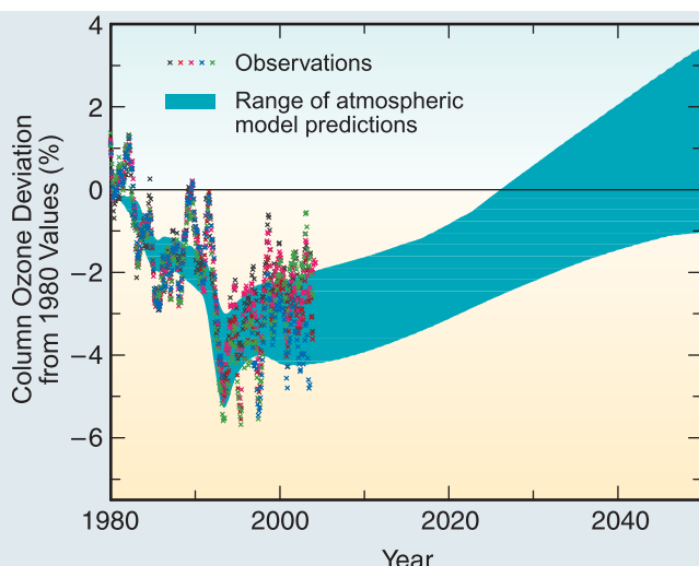
Figure TS-7. Observed and modelled changes in low- and mid-latitude (60°S – 60°N) de-seasonalised column ozone relative to 1980. The black symbols indicate ground-based measurements, and the coloured symbols various satellite-based data sets. The range of model predictions comes from the use of several different two-dimensional photochemistry models forced with the same halocarbon scenario; some models also allowed for the effect of changing CO 2 amounts on stratospheric temperatures. The measurements show that column ozone values between 60°S and 60°N decreased beginning in the early 1980s and the models capture the timing and extent of this decrease quite well. Modelled halogen source gas concentrations decrease in the early 21st century in response to the Montreal Protocol, so that simulated ozone values increase and recover towards pre-1980 values. [Box 1.7]
